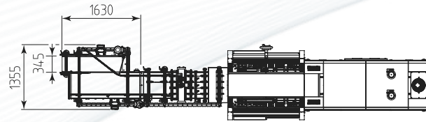
ALX flanked conveyor
