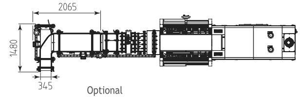
ALX 90° conveyor
